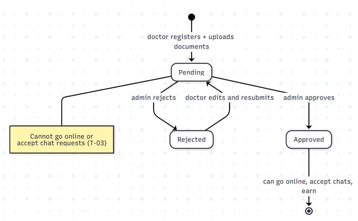
Fig-1: Doctor Registration
